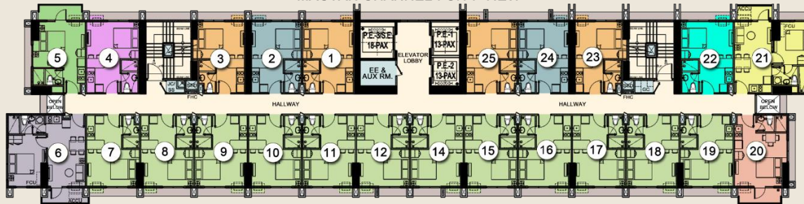
AMENITY VIEW TYP. 25TH - 30TH FLOOR PLAN
