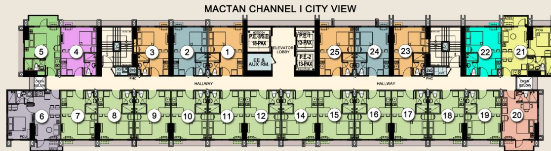
AMENITY VIEW TYP. 5TH - 12TH FLOOR PLAN
